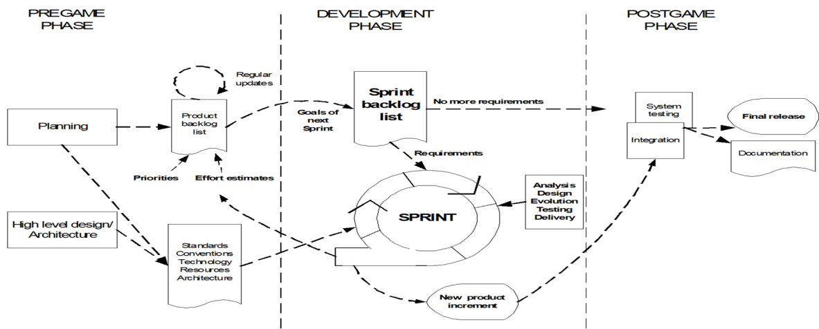
Fig 1: Scrum Process
